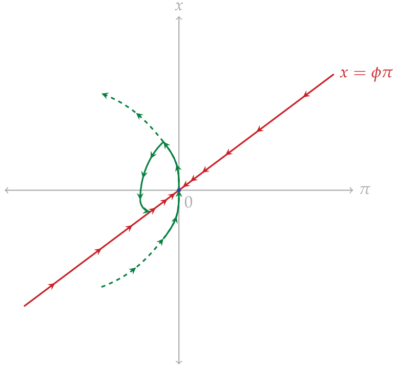
Figure 7: The optimum with the added constraint that \pi(t) \leq 0 for all t \geq 0 .
