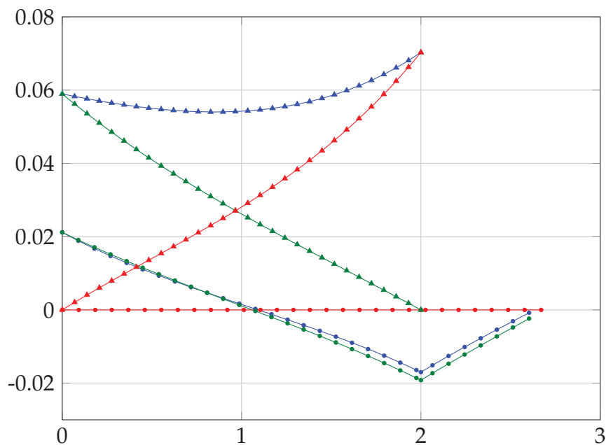
Figure 9: Total spending (blue), opportunistic spending (green) and stimulus spending (red) for a numerical example. Both the case with monetary commitment (circles) and discretion (triangles) are shown.
