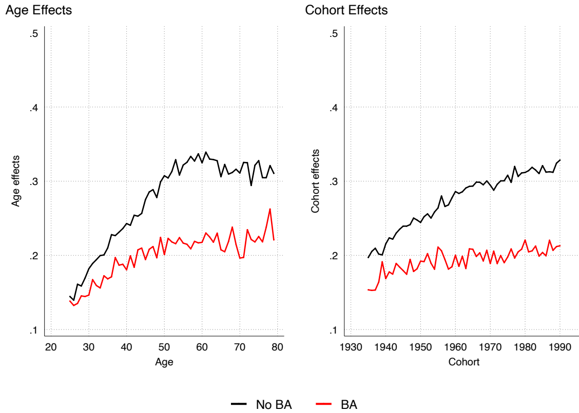
Figure S3: Age Effects and Cohort Effects (Replication of Case et al. 2020)
