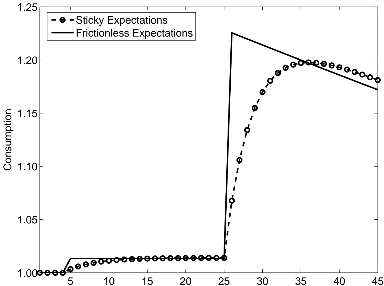
(a) Dynamics of the Consumption Ratio C
