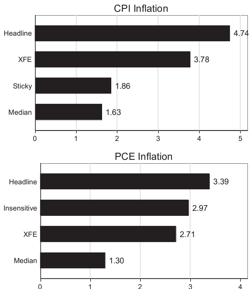
FIGURE 3 | Volatility of Monthly Annualised Inflation During 2020–21 (Standard deviation; percentage points). Note: “XFE” denotes inflation measure excluding food and energy. “Median” denotes weighted median series produced by the Federal Reserve Bank of Cleveland staff. “Insensitive” denotes series produced by Federal Reserve Bank of San Francisco staff (Shapiro 2020) that excludes food and energy as well as additional PCE components for which either prices or quantities moved in a statistically significant manner at the onset of the COVID-19 pandemic, between February and April 2020. “Sticky” denotes series produced by the Federal Reserve Bank of Atlanta staff based on a subset of CPI components assessed as slow to change due to the low frequency of price adjustment.
