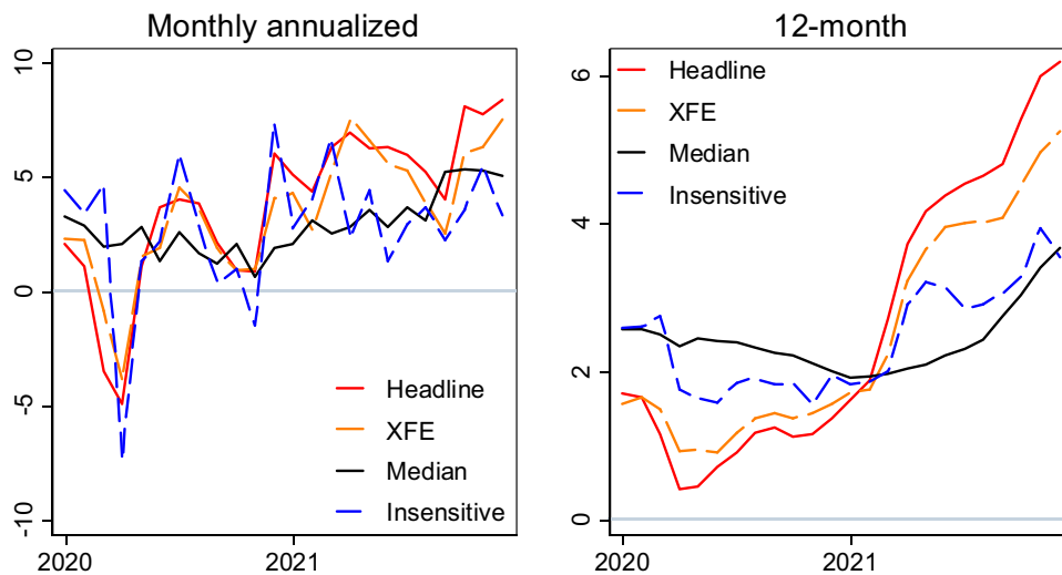
FIGURE 2 | Inflation Since COVID-19, 2020–2021 (percent). Note: “XFE” denotes inflation measure excluding food and energy. “Median” denotes weighted median series produced by the Federal Reserve Bank of Cleveland staff. “Insensitive” denotes series produced by Federal Reserve Bank of San Francisco staff (Shapiro 2020) that excludes food and energy as well as additional PCE components for which either prices or quantities moved in a statistically significant manner at the onset of the COVID-19 pandemic, between February and April 2020. “Sticky” denotes series produced by the Federal Reserve Bank of Atlanta staff based on a subset of CPI components assessed as slow to change due to the low frequency of price adjustment. [Color figure can be viewed at wileyonlinelibrary.com ]
