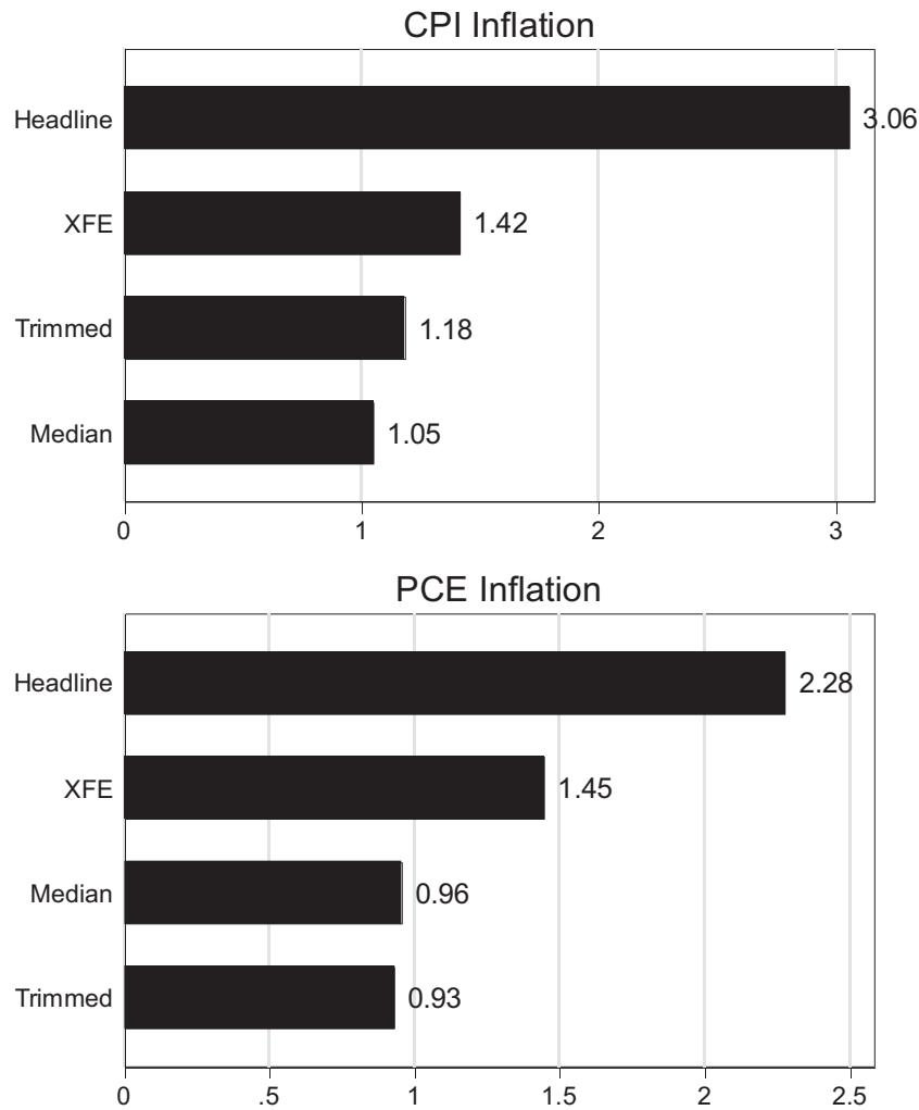
FIGURE 1 | Pre-pandemic Volatility of Monthly Annualised Inflation, 1985–2019 (Standard deviation; percentage points). Note: “XFE” denotes inflation measure excluding food and energy. “Median” denotes weighted median series produced by the Federal Reserve Bank of Cleveland staff. “Trimmed” denotes the trimmed mean series prepared by the Federal Reserve Bank of Cleveland staff and Federal Reserve Bank of Dallas staff for the CPI and PCE, respectively.
