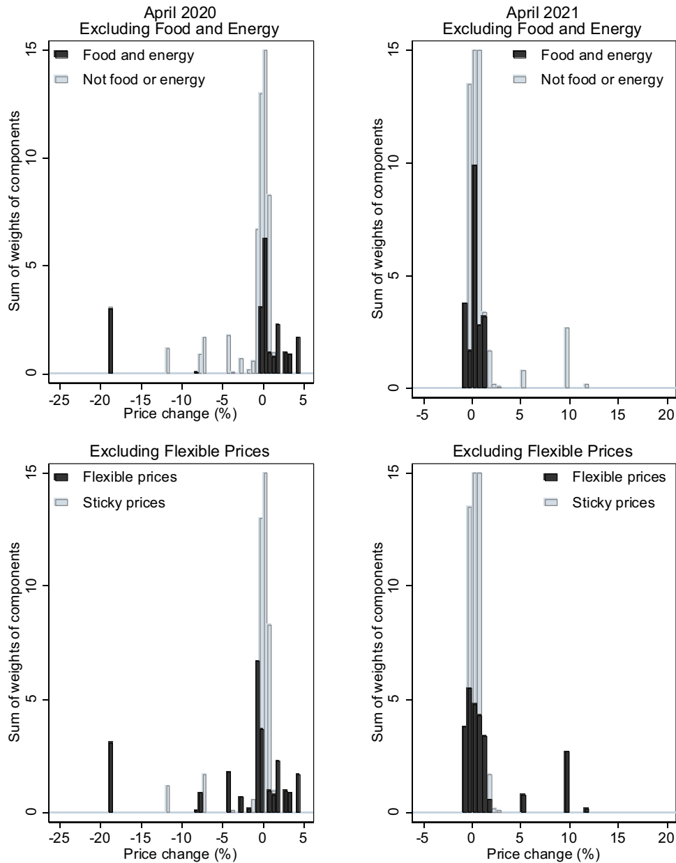
FIGURE 4 | April 2020 and April 2021: Histogram of Changes in the Prices of CPI Categories (Monthly, not annualised, percent). Note: Figure reports non-annualised inflation rates. Vertical axis cut off at 15. Weights computed following Dolmas (2005). “Flexible prices” refer to prices of industries that are excluded from the Federal Reserve Bank of Atlanta sticky-price CPI inflation measure.
