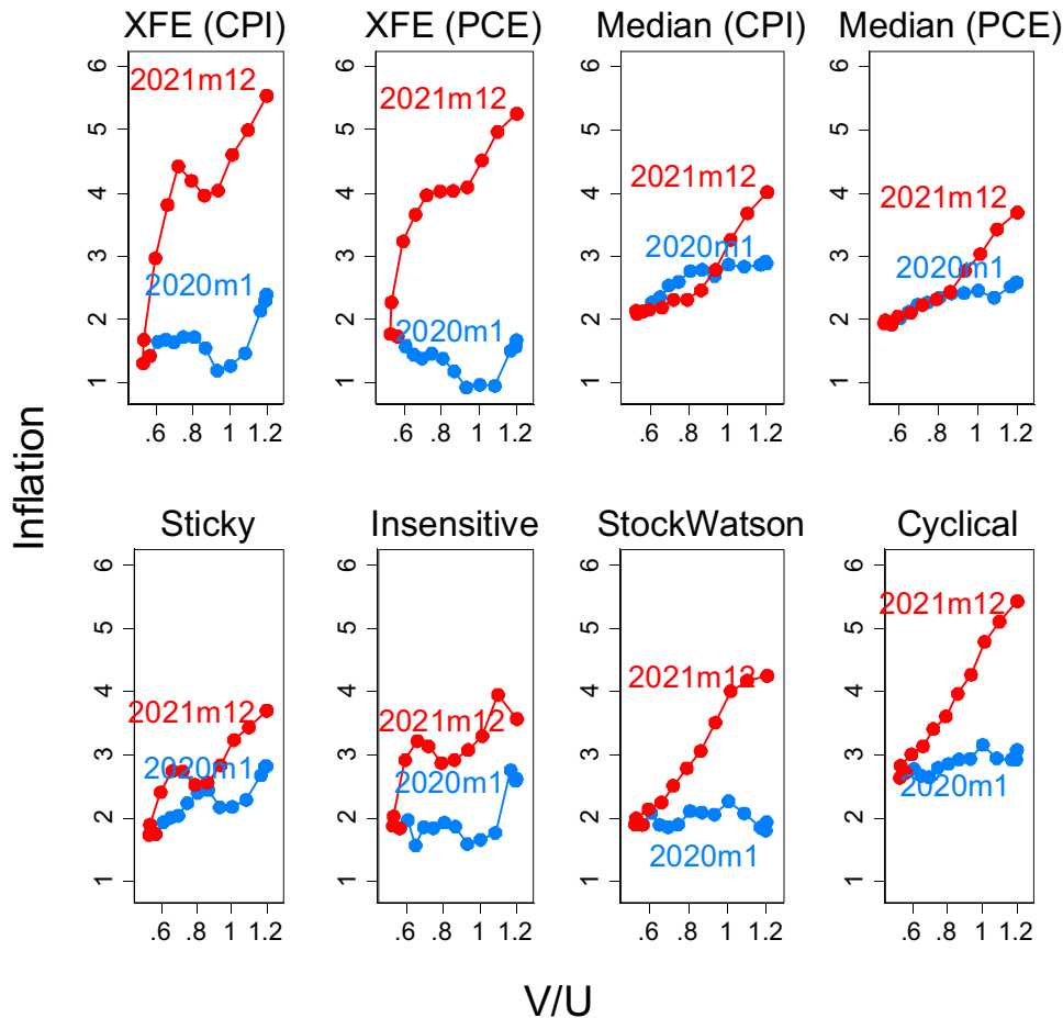
FIGURE 5 | Inflation Relation with Vacancy-to-unemployment Ratio, 2020–2021 (12-month rates; percent and ratio). Note: Blue points indicate 2020. Red dots indicate 2021. Inflation indicates 12-month inflation rate. V/U denotes the ratio of vacancies to unemployed (12-month average). “XFE” denotes CPI inflation measure excluding food and energy. “Median” denotes the weighted median CPI series produced by the Federal Reserve Bank of Cleveland staff. “Sticky” denotes a series produced by the Federal Reserve Bank of Atlanta staff based on a subset of CPI components assessed as slow to change due to the low frequency of price adjustment. “Insensitive” denotes the PCE series produced by the Federal Reserve Bank of San Francisco staff (Shapiro 2020) that excludes food and energy, as well as additional PCE components for which either prices or quantities moved in a statistically significant manner at the onset of the COVID-19 pandemic, between February and April 2020. “Cyclical” denotes the PCE measure produced by Federal Reserve Bank of San Francisco staff (Mahedy and Shapiro 2017) that excludes food and energy and also excludes additional items assessed as being acyclical. “StockWatson” denotes cyclically sensitive PCE inflation measure of Stock and Watson (2019) published on Federal Reserve Bank of Atlanta Underlying Inflation Dashboard. [Color figure can be viewed at wileyonlinelibrary.com ]
