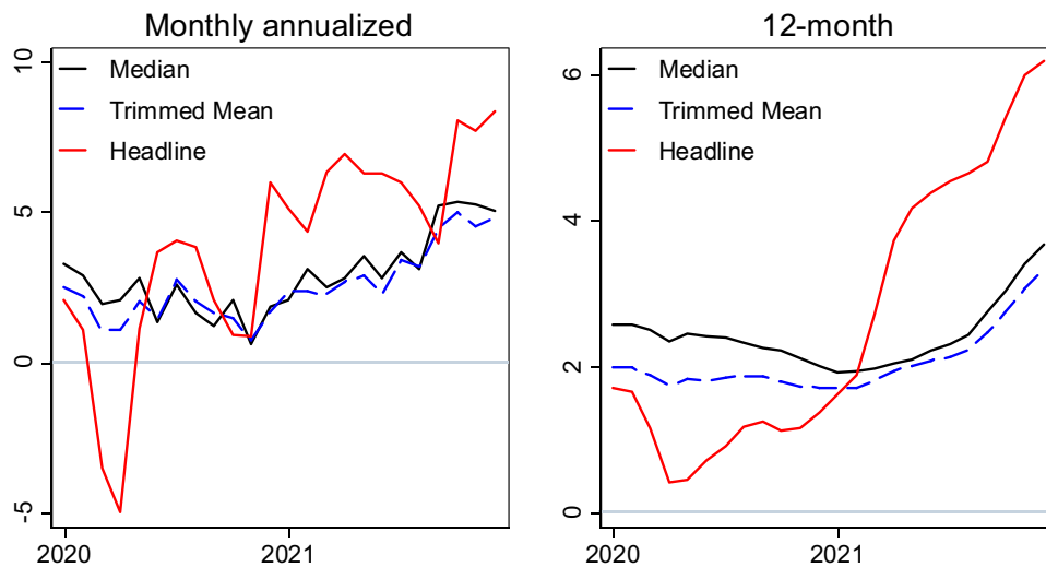
FIGURE 6 | Median and Trimmed-Mean Inflation, 2020–2021 (percent). Note: “Median” denotes weighted median series produced by the Federal Reserve Bank of Cleveland staff. “Trimmed” denotes the trimmed mean series prepared by the Federal Reserve Bank of Cleveland staff and Federal Reserve Bank of Dallas staff for the CPI and PCE, respectively. [Color figure can be viewed at wileyonlinelibrary.com ]
