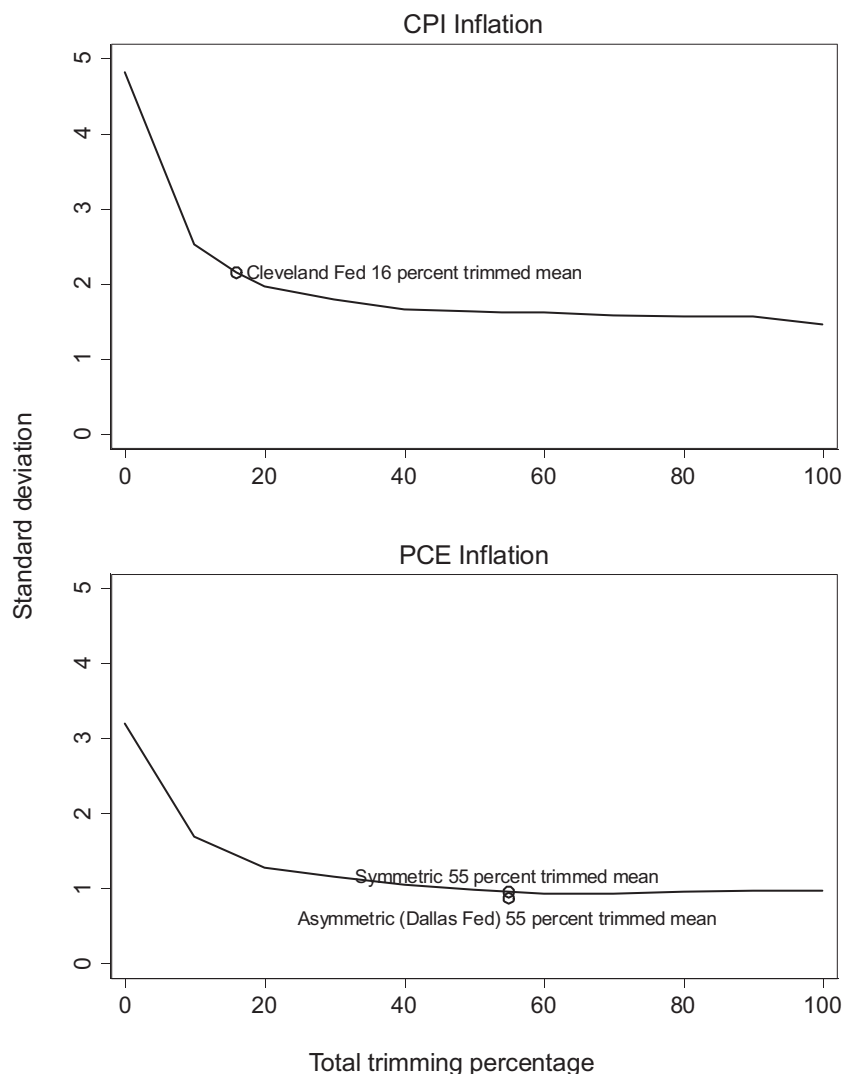
FIGURE 8 | Trimmed-mean inflation volatility versus total trimming percentage, 2020–2021 (Standard deviation of monthly annualised inflation; percentage points). Note: Total trimming percentage indicates the sum of the proportion of price changes trimmed from upper and from lower end of the weighted distribution of monthly price changes.
