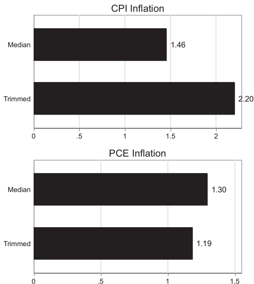
FIGURE 7 | Volatility of median and trimmed-mean monthly annualised inflation during 2020–2021 (Standard deviation; percentage points). Note: “Median” denotes the weighted median series produced by the Federal Reserve Bank of Cleveland staff. “Trimmed” denotes the trimmed mean series prepared by the Federal Reserve Bank of Cleveland staff and Federal Reserve Bank of Dallas staff for the CPI and PCE, respectively.
