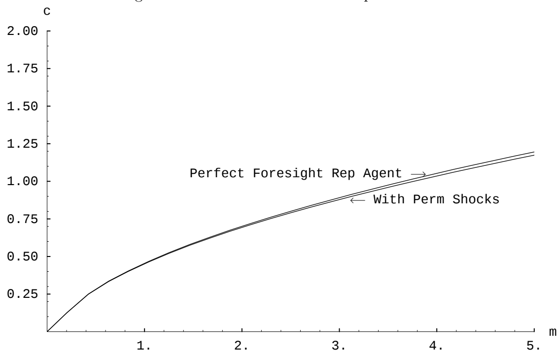
Figure 1: Macro and Micro Consumption Functions
