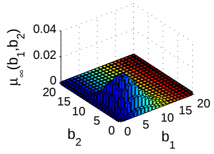
Limit distribution ( \theta = 2, \lambda = 1 )
