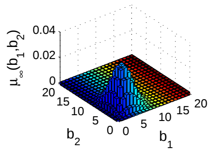
Limit distribution ( \theta = 3, \lambda = 0 )
