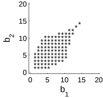
Compatibility ( \theta = 3, \lambda = 1 )
