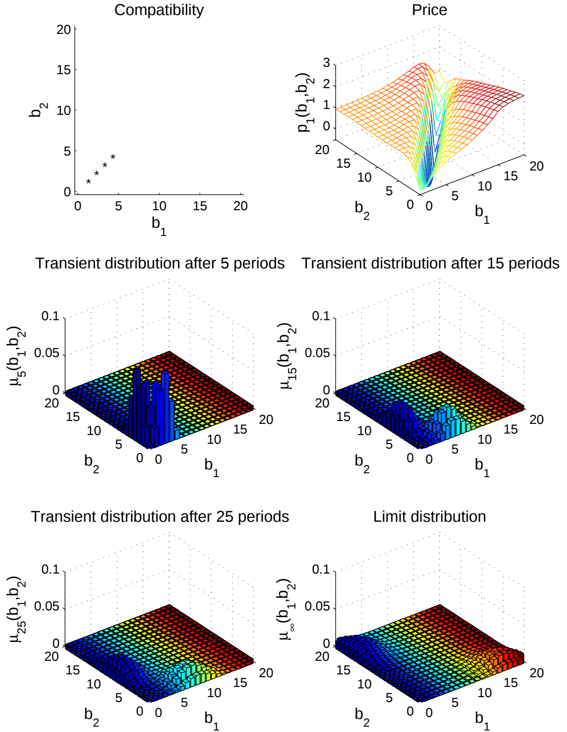
Figure 2: Tipping equilibrium. Compatibility (a * indicates compatible products) and price, transient and limit distribution. \theta = 3 , \lambda = 1 , \delta = .06 .
