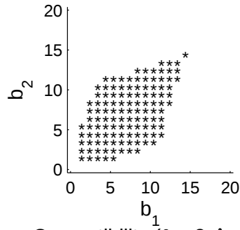
Compatibility ( \theta = 3, \lambda = 0 )
