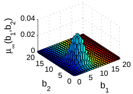
Limit distribution ( \theta = 3, \lambda = 1 )
