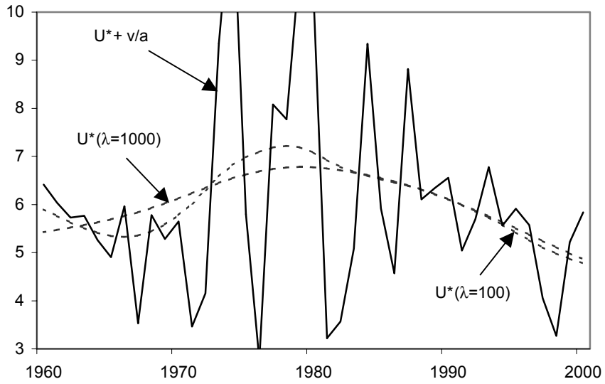
Figure 1 Time-Varying NAIRUs, 1960-2000
