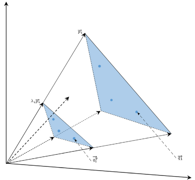
Fig. 1. Eigenvalue-eigenvector decomposition in the 2.1-measurement model.
