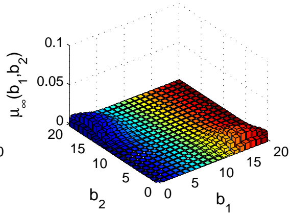
Limit distribution
