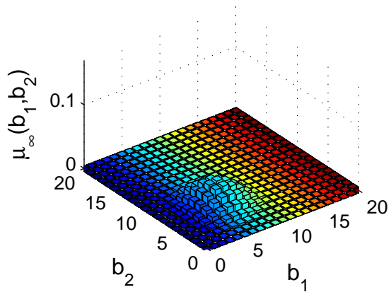
Limit distribution
